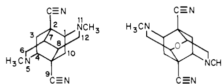
Chart I. 2,9-Dicyano-5,11-dimethyl-5,11-diazatetracyclo[6.2.2.0 2,7 .0 4,9 ]dodecane ( 1 ) a
